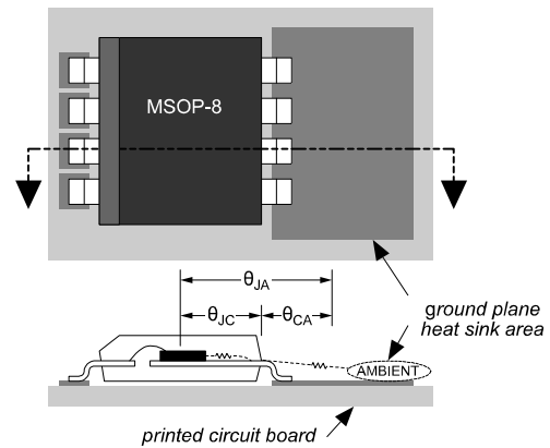
Figure 5. Thermal Resistance
