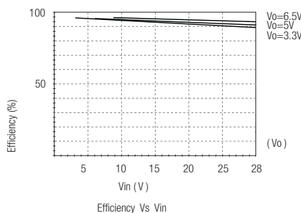
R-74xx Efficiency VS Vin
