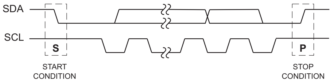
Figure 50. Bit Transfer
