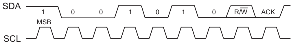
Figure 52. Slave Address
