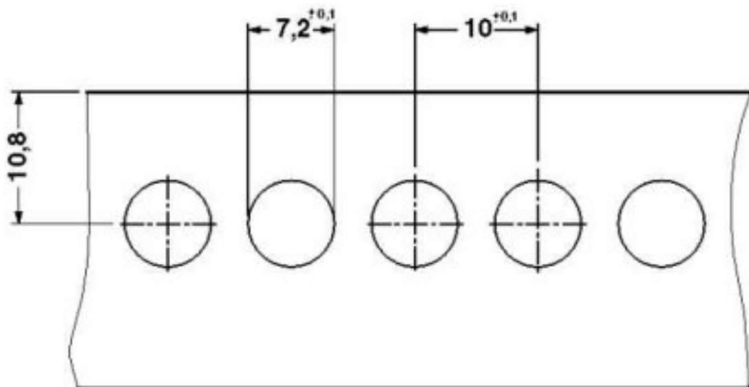
Drilling diagram
