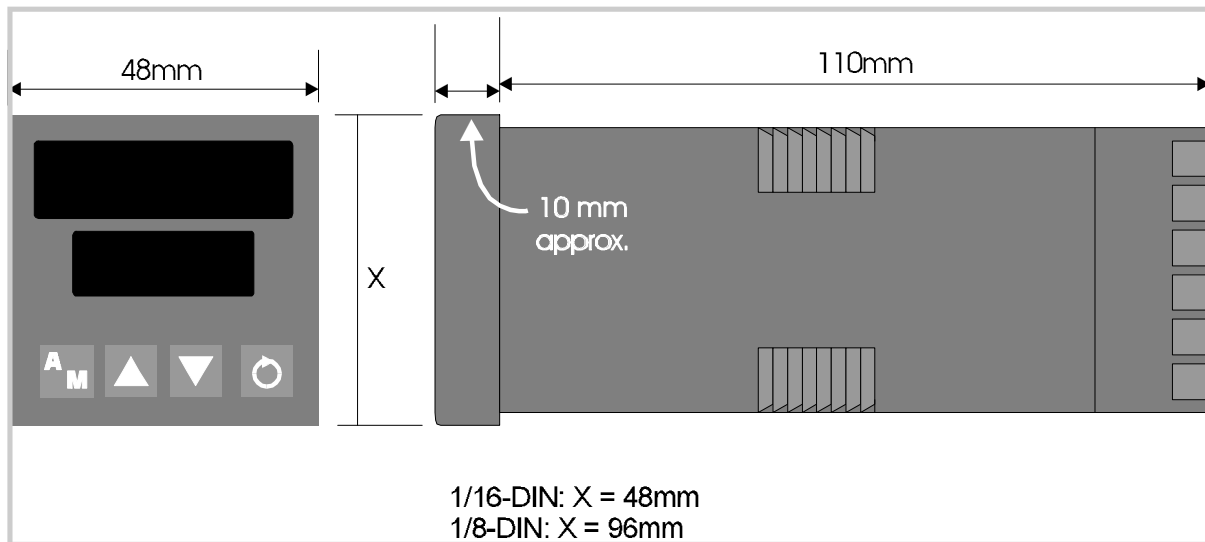
Figure 1-2 Main Dimensions
