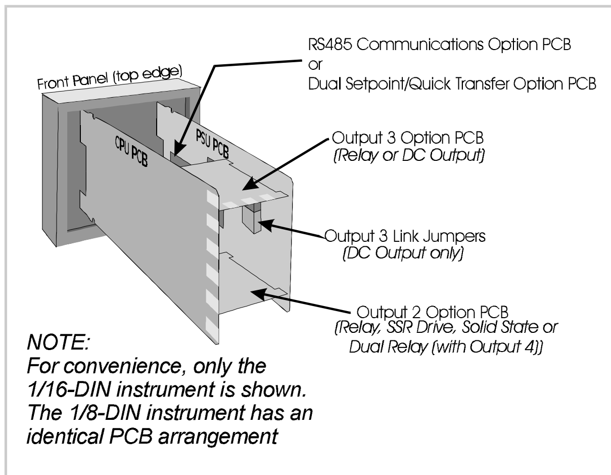
Figure 2-1 PCB Positions
