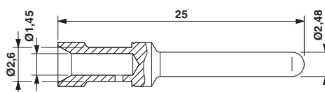
Dimensioned drawing
