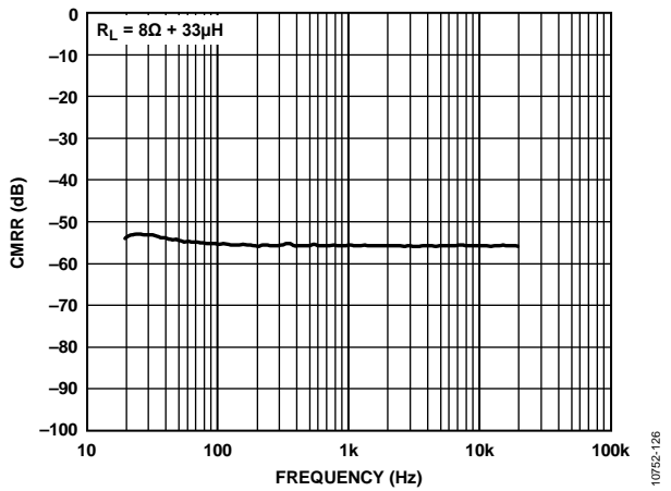
Figure 26. Common-Mode Rejection Ratio (CMRR) vs. Frequency, PVDD = 5 V, RL = 8 Ω
