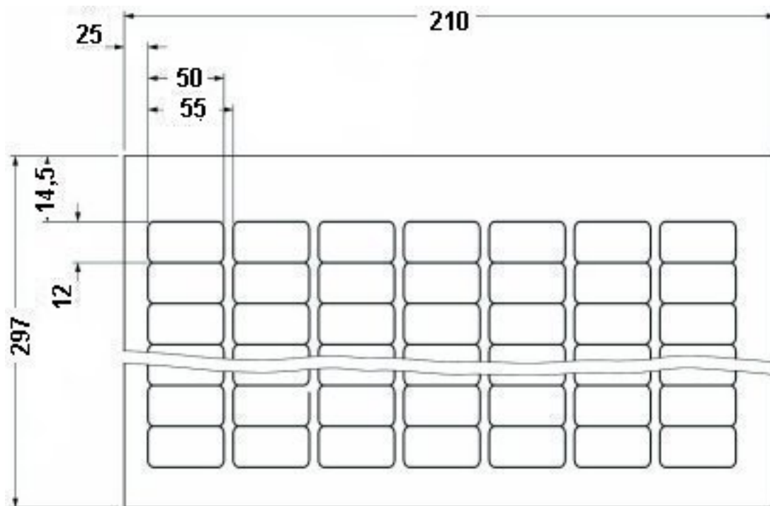
Dimensioned drawing
