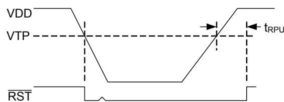
Figure 2. Low Voltage Reset
