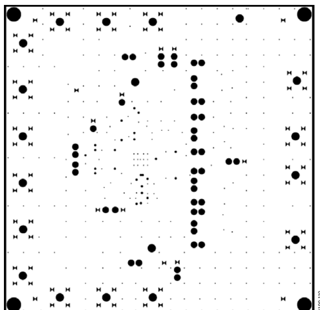
Figure 119. Inner Layer 1
