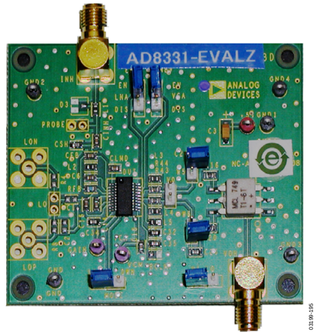
Figure 95. AD8331-EVALZ Top View
