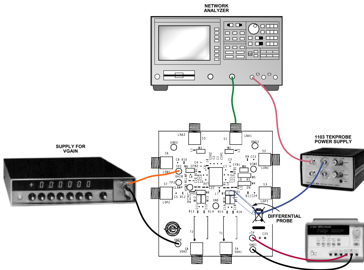
Figure 106. AD8332—Typical Board Test Connections
