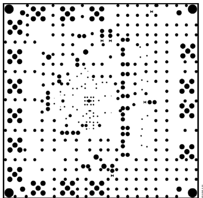
Figure 120. Inner Layer 2
