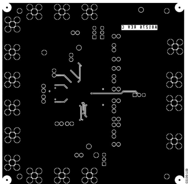
Figure 118. Wiring Side Copper
