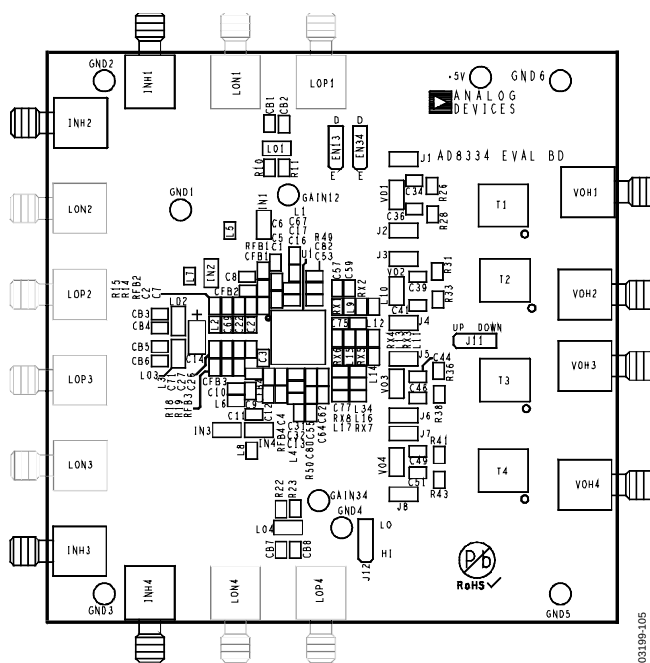
Figure 114. AD8334-EVALZ Assembly
