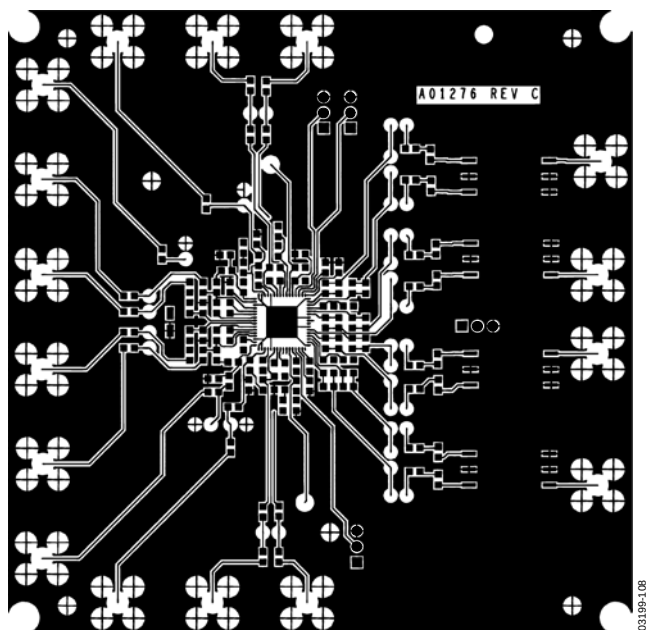
Figure 117. Component Side Copper
