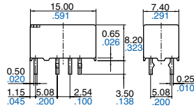
Self clinching terminal
