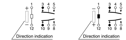
Schematic (Bottom view) Single side stable 1 coil latching
