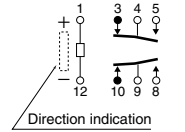
Schematic (Bottom view) Single side stable 1 coil latching
