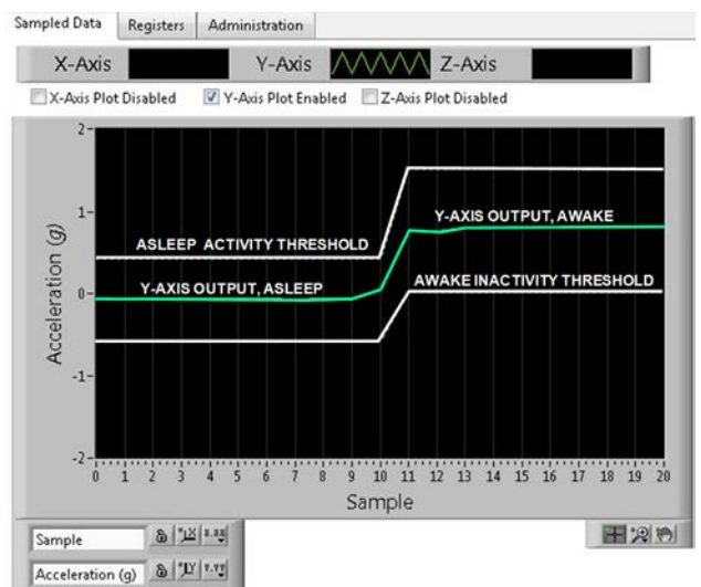
Figure 2. Screen Shot of Evaluation Software Output
