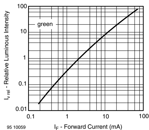
Fig. 16 - Relative Luminous Intensity vs. Forward Current
