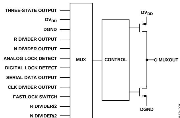
Figure 15. MUXOUT Schematic
