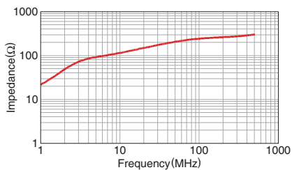
HF56RH14.3X28.6X6.35
