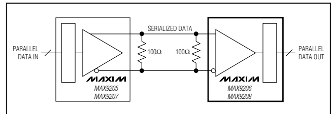
Figure 10. Double-Termination Point-to-Point
