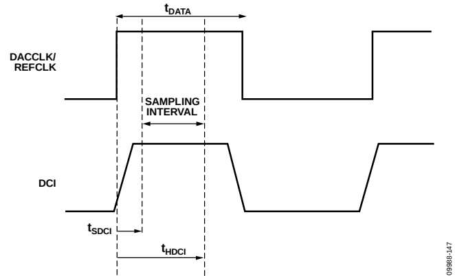
Figure 84. Timing Diagram for Input Data Port (Data Rate Mode)
