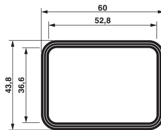
Dimensioned drawing
