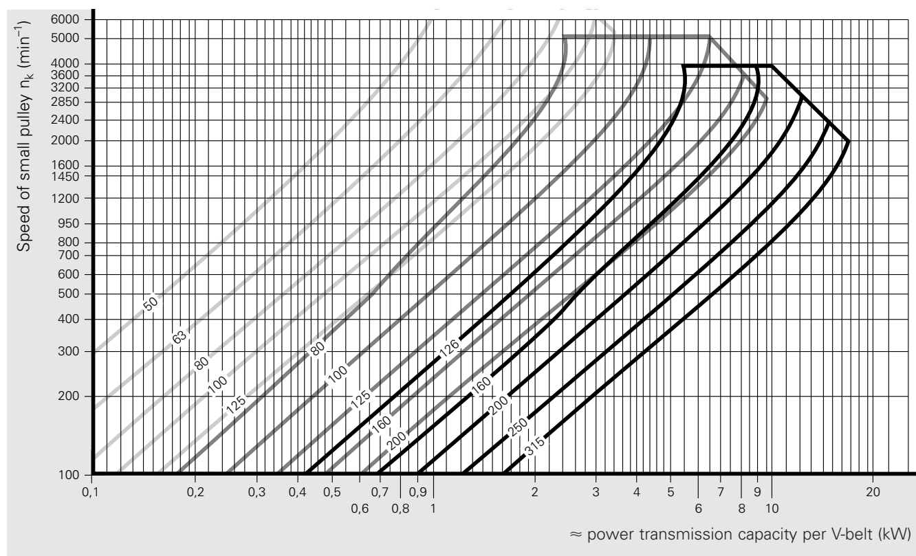
CONTI MULTIFLEX® classical-section wrapped V-belts 22/C — 32/D — 40/E —
