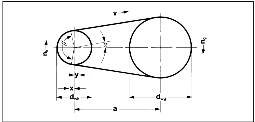
Two-pulley drive
