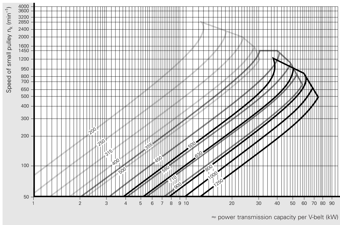
CONTI MULTIFLEX® classical-section wrapped V-belts 22/C — 32/D — 40/E —
