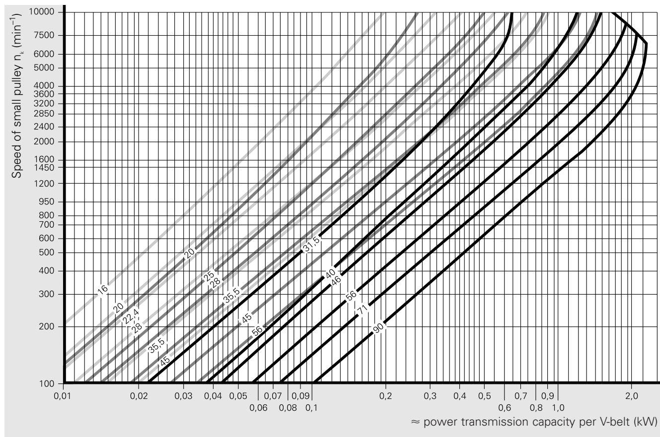
CONTI FO®-Z heavy-duty cogged raw edge V-belts 5 — 6 — 8 —
