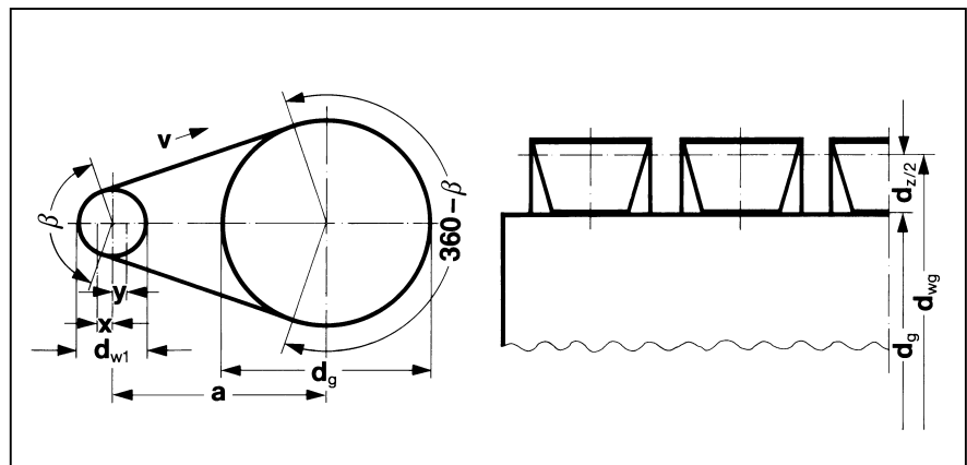
V-flat drive
