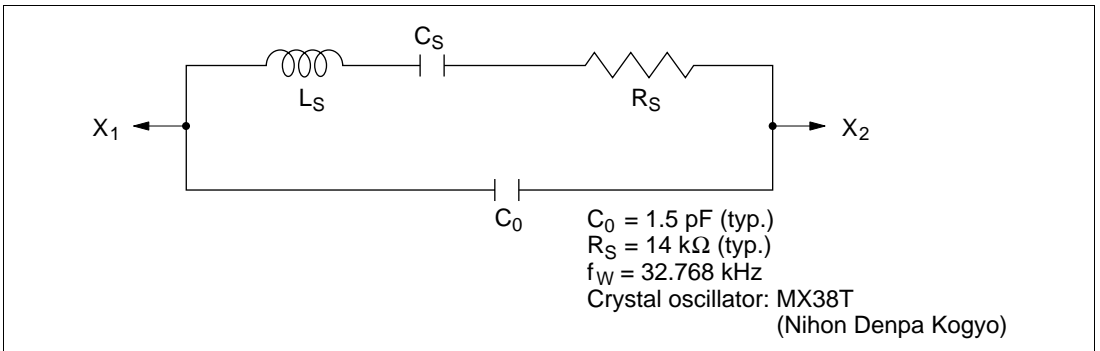
Figure 4.8 Equivalent Circuit of 32.768-kHz Crystal Oscillator
