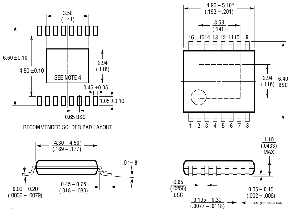
FE Package 16-Lead Plastic TSSOP (4.4mm) (Reference LTC DWG # 05-08-1663) Exposed Pad Variation BC
