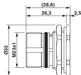
Dimensioned drawing
