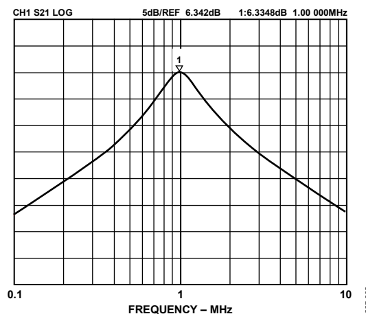
Figure 68. Band-Pass Filter Response
