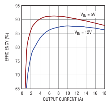
1.2V OUT Efficiency vs I OUT
