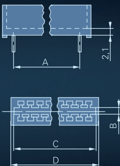
Without flange
