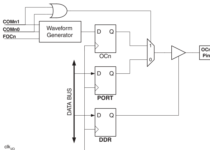
Figure 56. Compare Match Output Unit, Schematic
