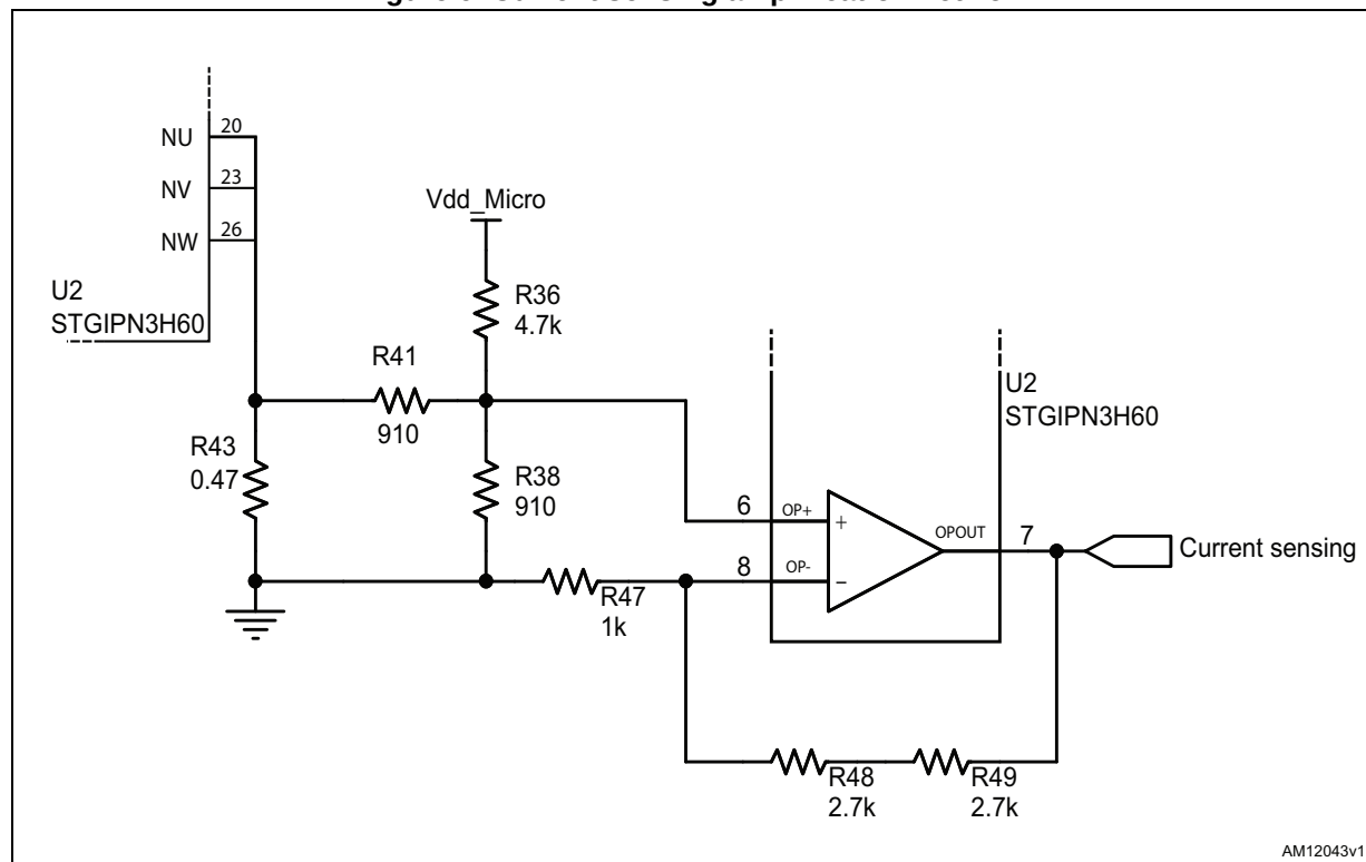
Figure 9. Current sensing amplification network
