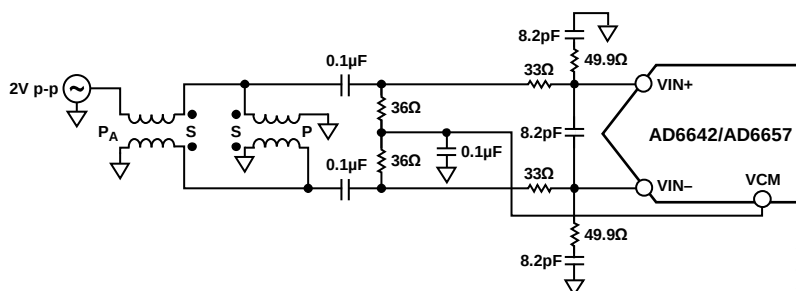
Figure 3. Default Analog Input Configuration of the AD6642/AD6657
