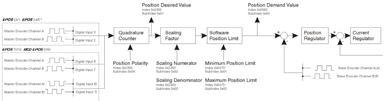
Figure 1: System Structure
