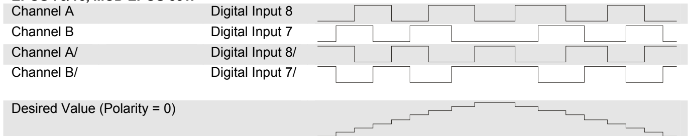
Figure 3: Quadrature Counter
