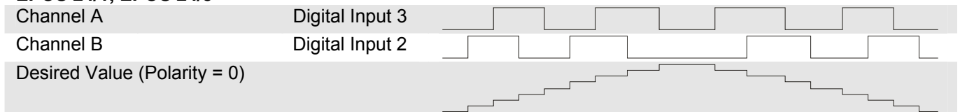
Figure 2: Quadrature Counter
