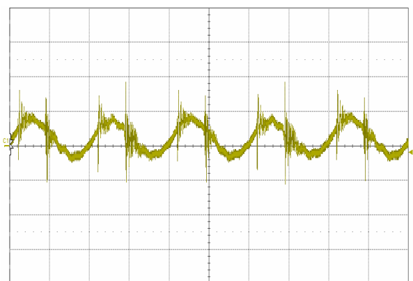
Figure 9. Output voltage ripple (20 mV/div.) at full rated load current into a resistive load with C_o = 10\mu\text{F} tantalum + 1 \mu\text{F} ceramic and V_{in} = 48\text{V} . Time scale: 1 \mu\text{s} /div.
