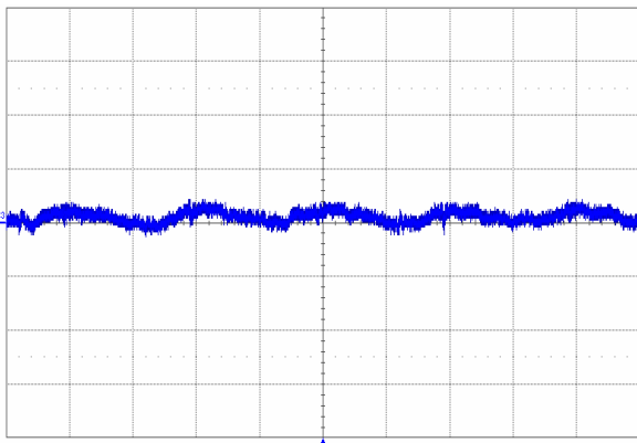
Figure 11. Input reflected-ripple current, i_s (20 mA/div.), measured through 10 \mu H at the source at full rated load current and V_{in} = 48 V. Refer to Figure 10 for test setup. Time scale: 1 \mu s/div.
