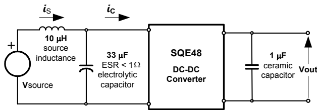
Figure 10. Test setup for measuring input reflected ripple currents, i_c and i_s .
