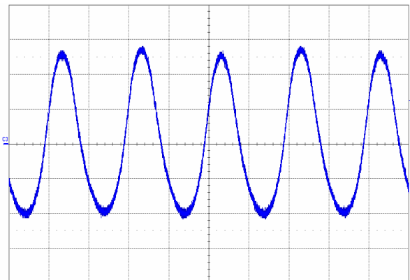
Figure 12. Input reflected-ripple current, i_c (100 mA/div.), measured at input terminals at full rated load current and V_{in} = 48 V. Refer to Figure 10 for test setup. Time scale: 1 \mu s/div.
