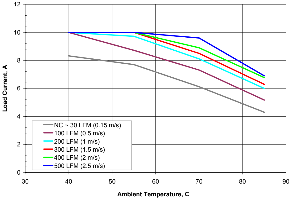
Figure 1. Available load current vs. ambient air temperature and airflow rates for SQE48T10120 converter mounted vertically with air flowing from pin 3 to pin 1, MOSFET temperature \leq 120^{\circ}\text{C} , V_{in} = 48\text{ V} .
