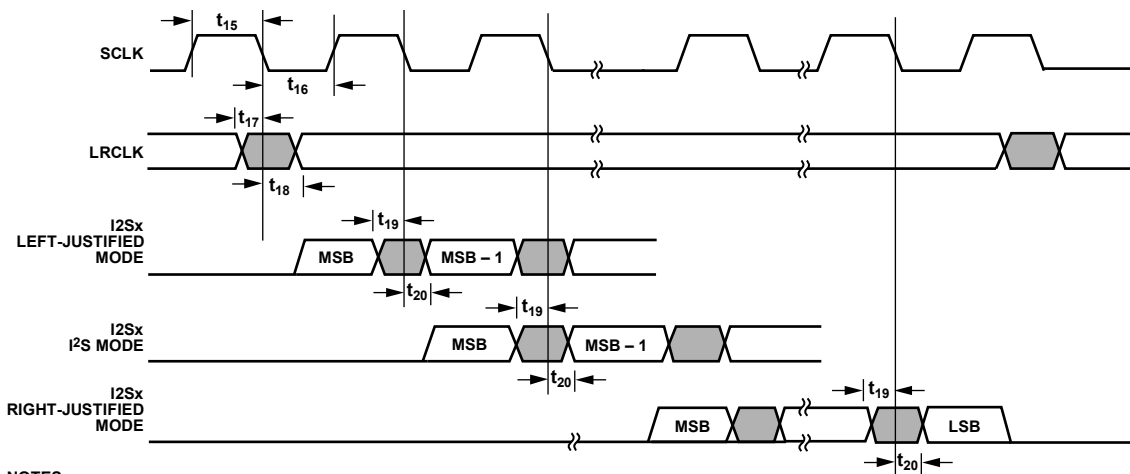
Figure 5. I²S Timing
