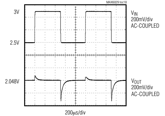
LINE-TRANSIENT RESPONSE ( V_{OUT} = 2.048V )
