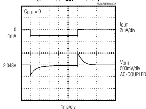
LOAD-TRANSIENT RESPONSE (SINKING, V_{OUT} = 2.048V )
