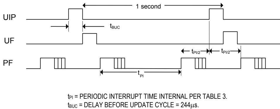
Figure 4. Update-Ended And Periodic-Interrupt Relationship
