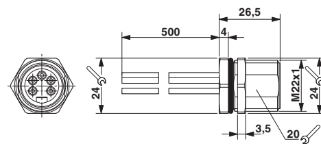
7/8" flush-type plug
