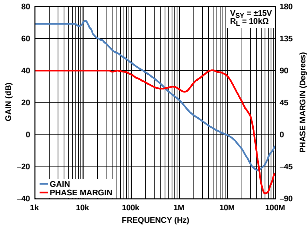
Figure 15. Gain and Phase Margin vs. Frequency, T_A = 210^\circ C
