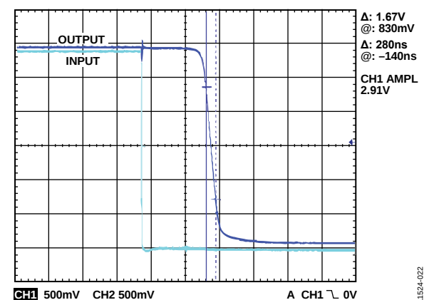
Figure 20. Large Signal Negative Edge Response, V_{SV} = \pm 15.0V , T_A = 210^\circ C
