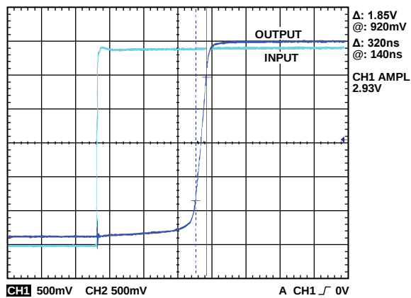
Figure 16. Large Signal Positive Edge Response, V_{SV} = \pm 15.0V , T_A = 175^\circ C
