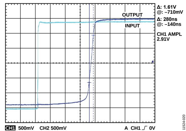
Figure 19. Large Signal Positive Edge Response, V_{SV} = \pm 15.0V , T_A = 210^\circ C
