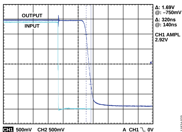
Figure 17. Large Signal Negative Edge Response, V_{SV} = \pm 15.0V , T_A = 175^\circ C
