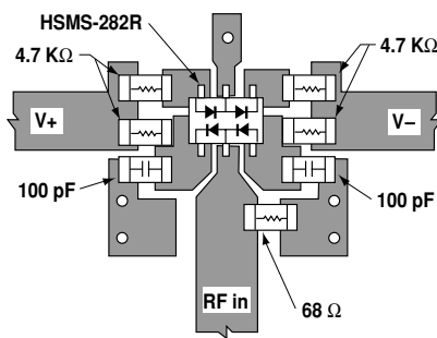
Figure 20. Layout of Suppressed Harmonic Detector.
