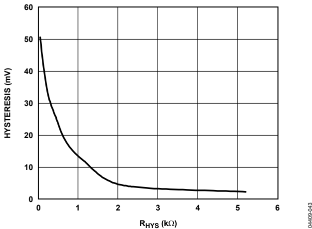
Figure 7. Hysteresis vs. R_{HYS} Control Resistor
