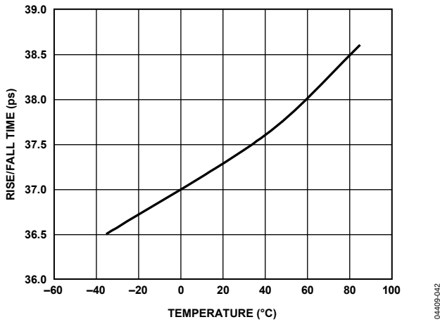
Figure 6. Rise/Fall Time vs. Temperature
