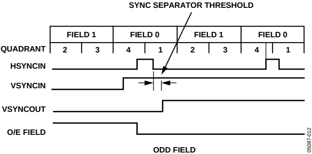
Figure 12. Vsync Filter—Odd/Even
