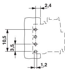
Drilling diagram
