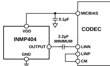
Figure 6. INMP404 Connected to a Codec
