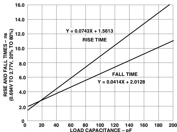
Figure 43. Typical Output Rise/Fall Time (20% - 80%, V_{DDEXT} = \text{Max} )
