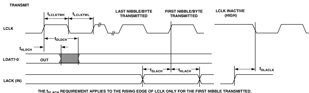
Figure 32. Link Ports—Transmit
