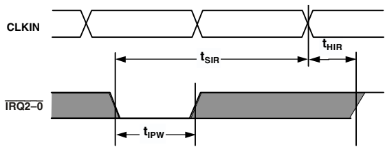
Figure 18. Interrupts
