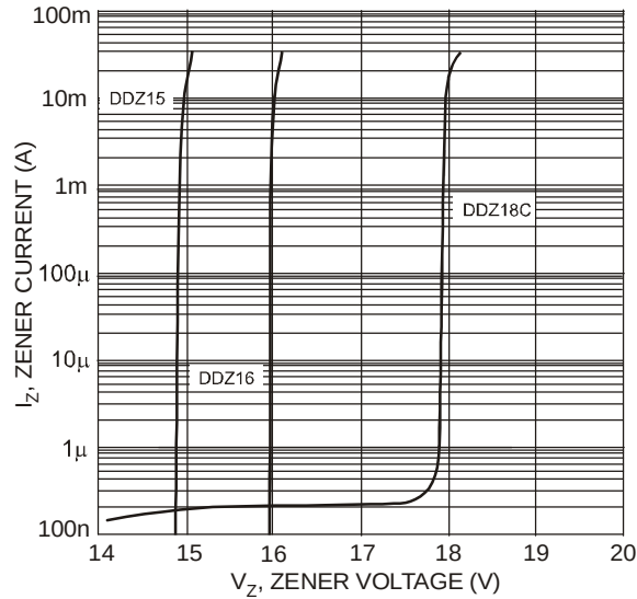
Fig. 6 Typical Zener Breakdown Characteristics, DDZ15 - DDZ18C
