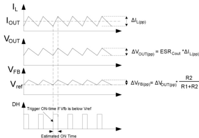
Figure 2. MIC26400 Control Loop Timing
