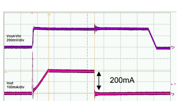
Reverse-Current Limit
