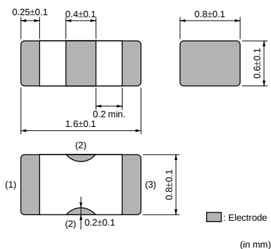
NFM18PC (0.1 to 0.47 \mu F, 2.2 \mu F-6.3V)
