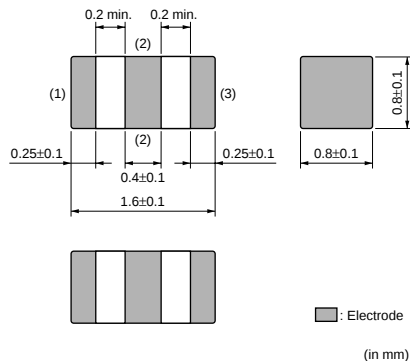
NFM18PC (1 \mu F, 2.2 \mu F-10V)
