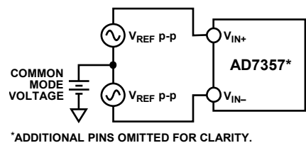
Figure 19. Differential Input Definition
