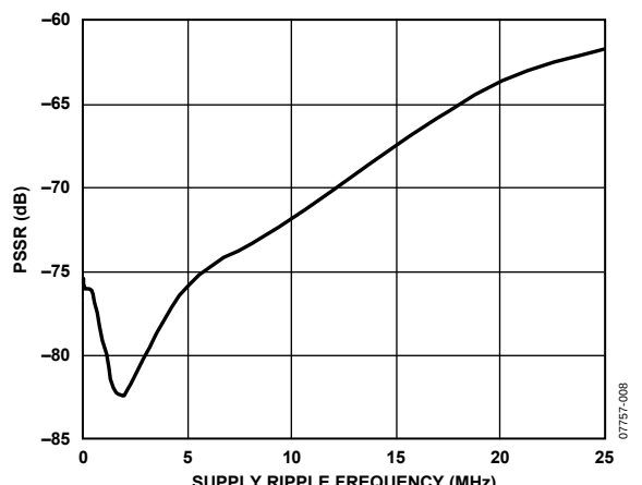
Figure 8. PSRR vs. Supply Ripple with No Supply Decoupling
