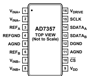
Figure 2. Pin Configuration
