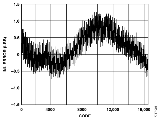
Figure 5. Typical INL
