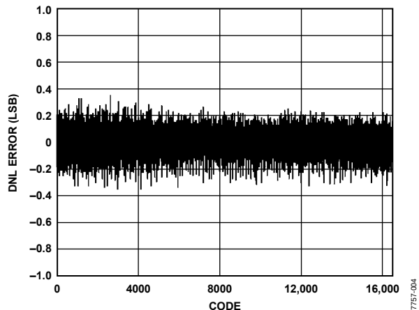
Figure 4. Typical DNL
