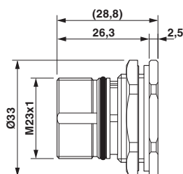
Dimensioned drawing
