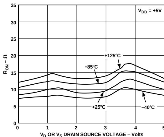
Figure 3. On Resistance as a Function of V_D ( V_S ) for Different Temperatures V_{DD} = 5\text{ V} (A Grade)
