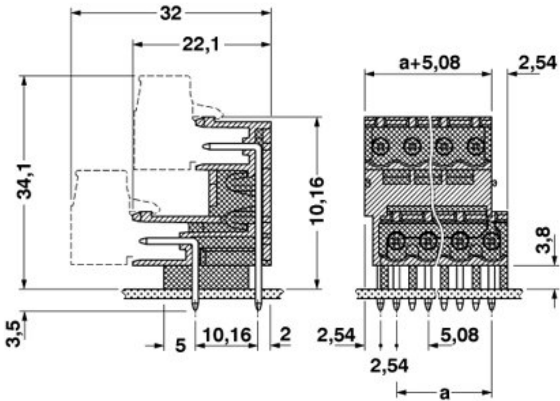
Dimensioned drawing
