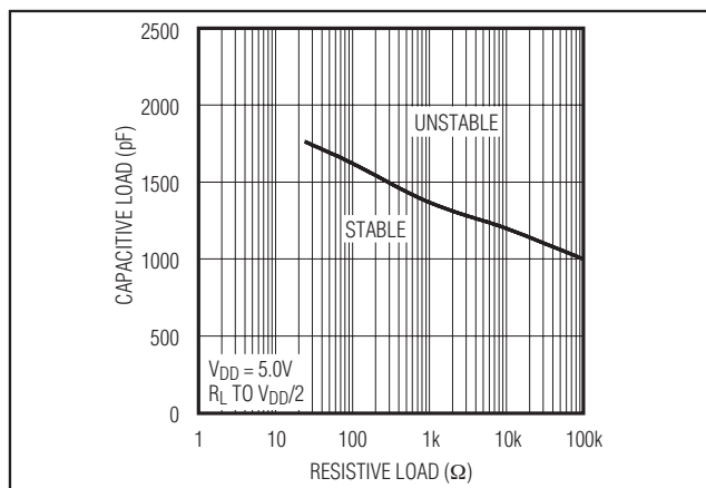
Figure 6. Capacitive-Load Stability
